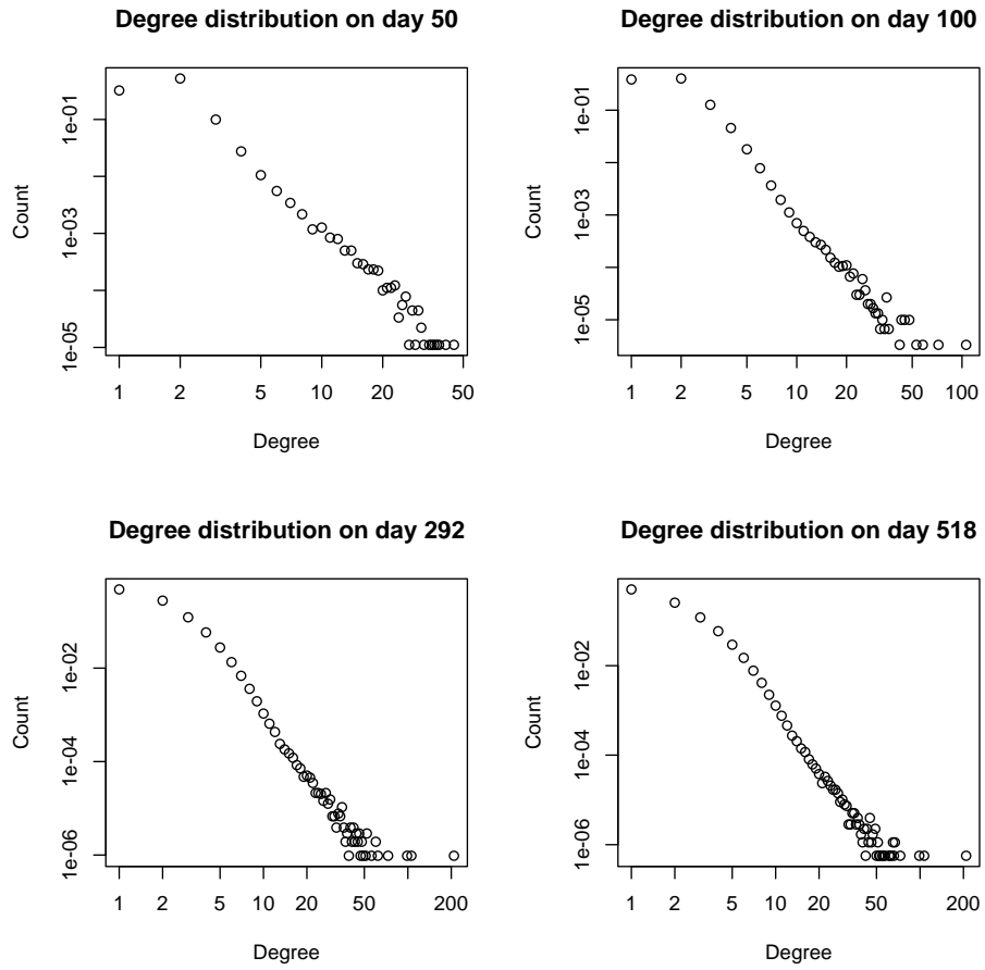
Fig. 2. The recruitment graph: Degree distributions over time. All plots are on log-log scale. Days 292 and 518 correspond to February 17th, 2016 and September 30th, 2016, respectively.
