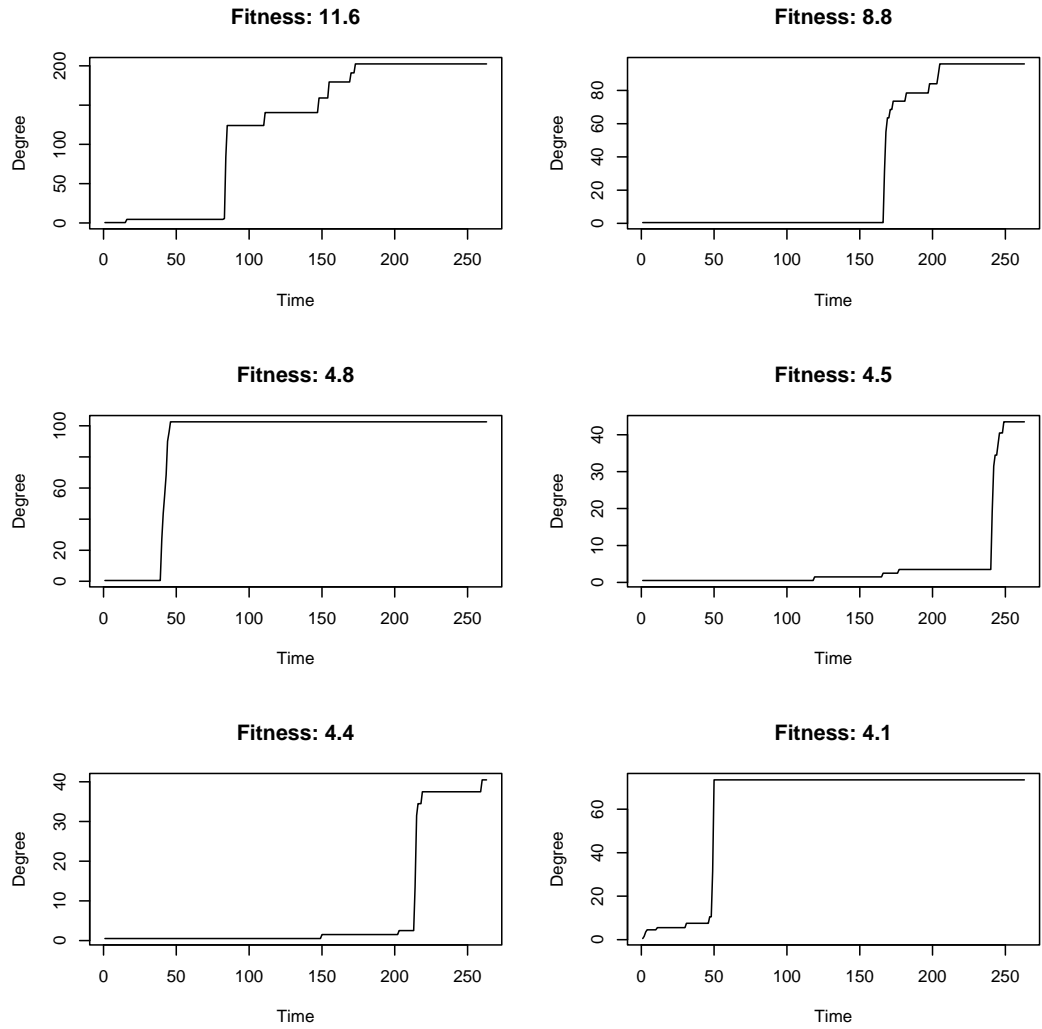
Fig. 6. Degree growth curves for selected nodes with high estimated fitness.
