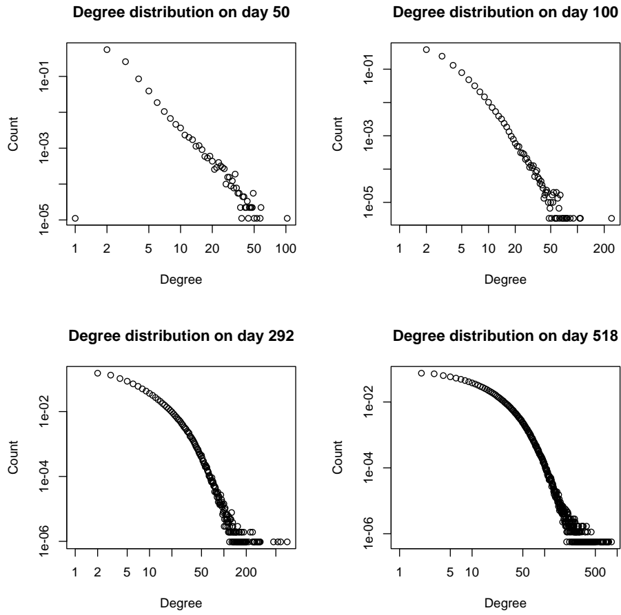
Fig. 3. The friends graph: Degree distributions over time. All plots are on log-log scale. Days 292 and 518 correspond to February 17th, 2016 and September 30th, 2016, respectively.
