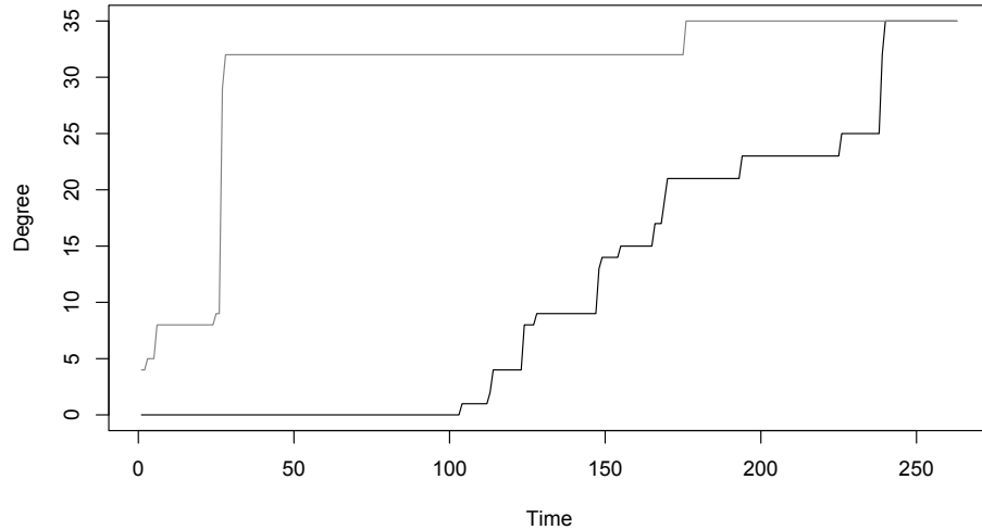
Fig. 8. Degree growth curves for two nodes with fitnesses equal to 3.61 (black) and 2.06 (grey), respectively.
