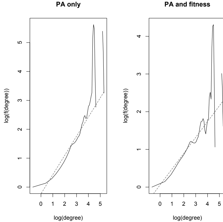
Fig. 4. Left: The estimated f(d) -function assuming that all fitnesses are one. Right: The estimated f(d) -function when the fitness effect is taken into account. Both plots are on a log-log scale.
