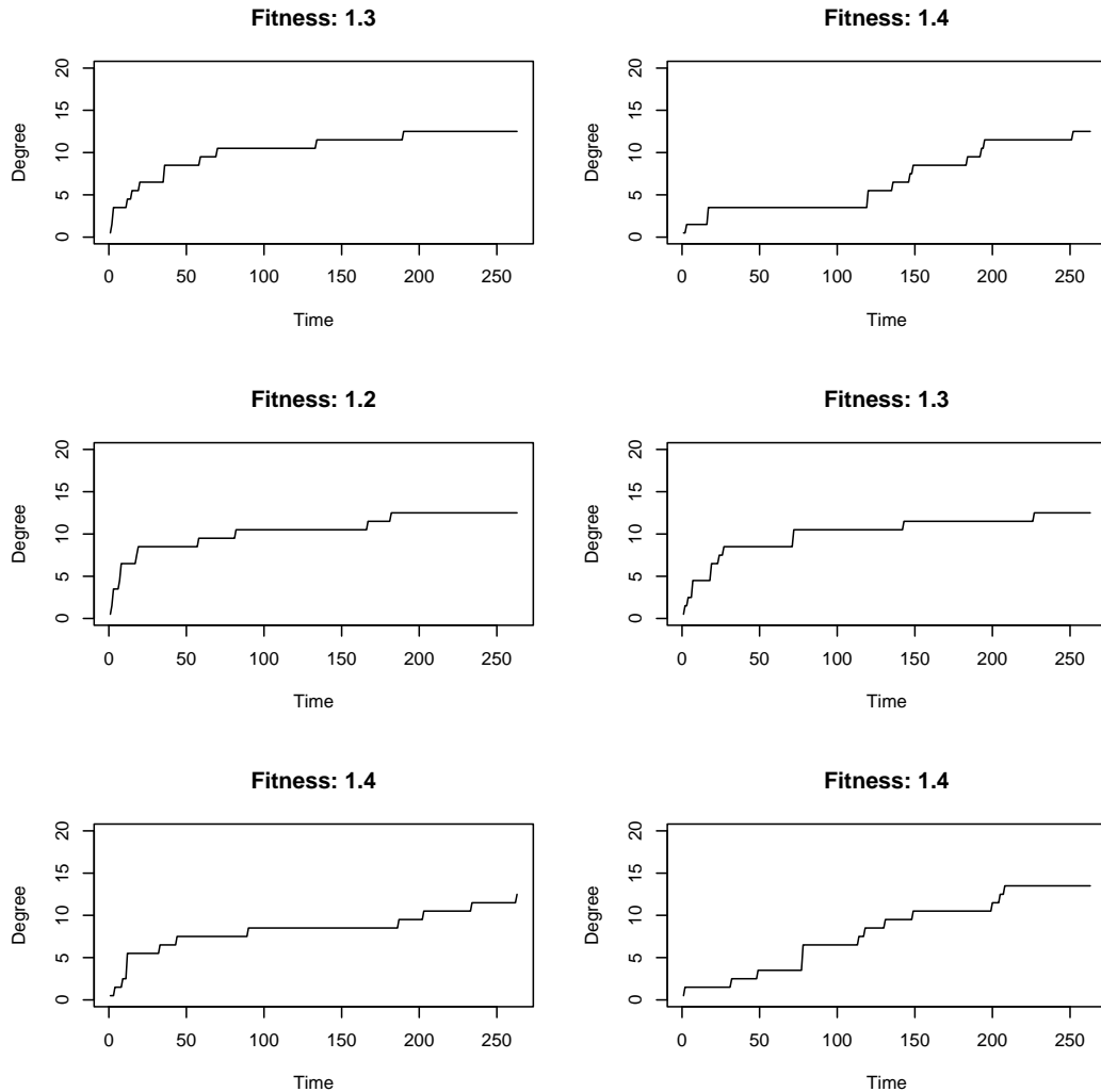
Fig. 7. Degree growth curves for selected nodes with low estimated fitness.
