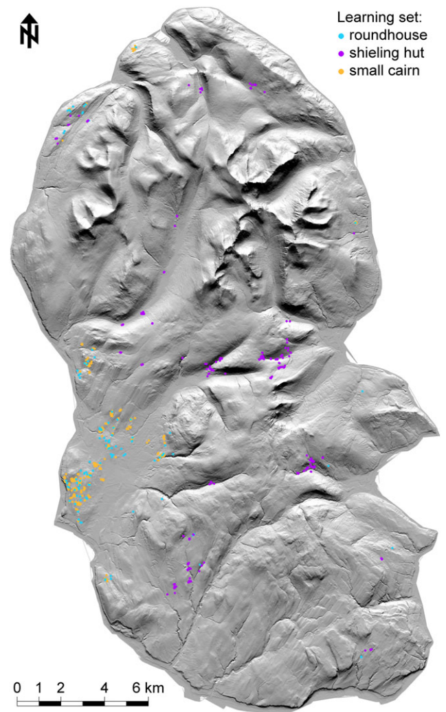
FIGURE 1 Hillshade relief visualization of the digital terrain model (DTM) of Arran, illustrating the complex topography of the island. The learning set locations are superimposed. DTM derived from airborne laser scanning (ALS). The DTM contains public sector information licensed under the Open Government Licence v3.0. [Colour figure can be viewed at wileyonlinelibrary.com ]
