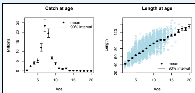
Estimated catch-at-age and length-at-age with 90% confidence intervals for cod.
