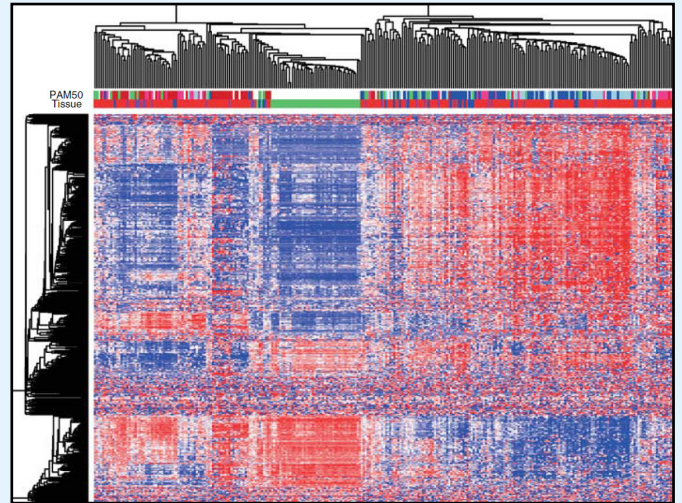
Hierarchical clustering of the methylation level of the 500 most variable gene regions.
