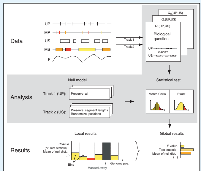
Flow diagram of the mathematics of genomic tracks.
