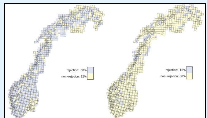
Discrepancies between downscaled reanalysis precipitation and gridded observations (autumn). Spatially independent two-sample statistical tests reported as the fraction of grid cells rejected for uncalibrated (left panel) and calibrated (right panel) reanalysis out of sample test data.
