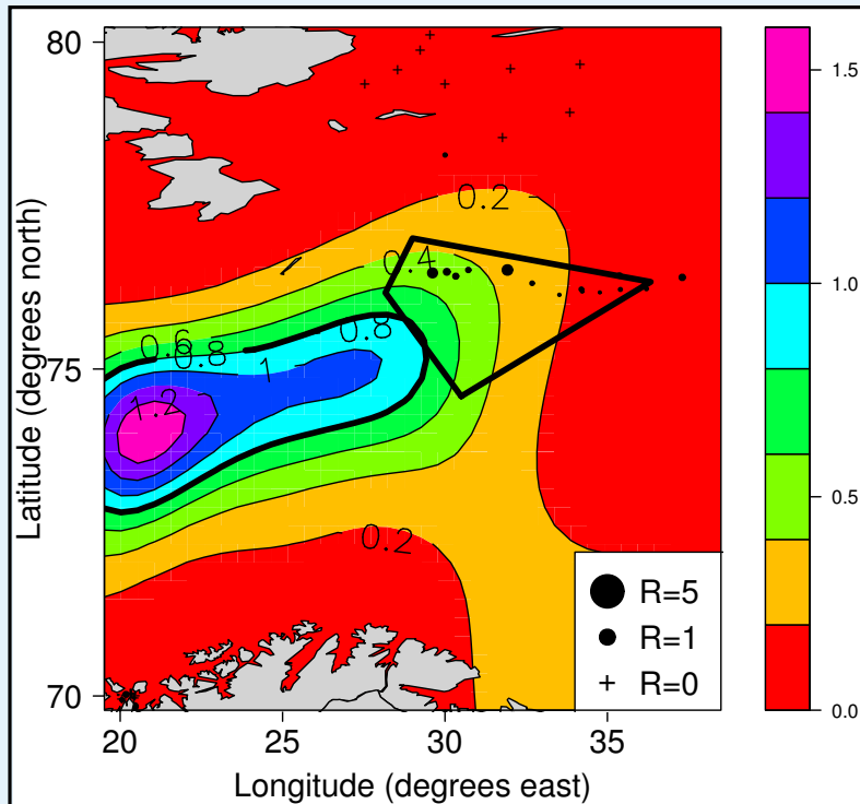
Contour plots of the estimated bycatch ratio. Circle areas are proportional to the bycatch ratios. Samples with zero bycatch rates are marked with a " + " symbol.
