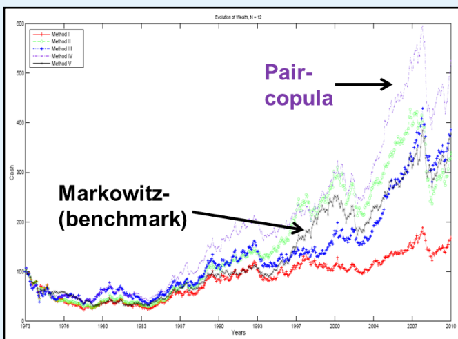
The accumulation of wealth if 100 $ is invested in a portfolio consisting of 12 American industry indices in 1973 and then rebalanced every month using 5 different strategies. The strategy that is based on the pair-copula construction outperforms its competitors. Source: University of Queensland Business School.
