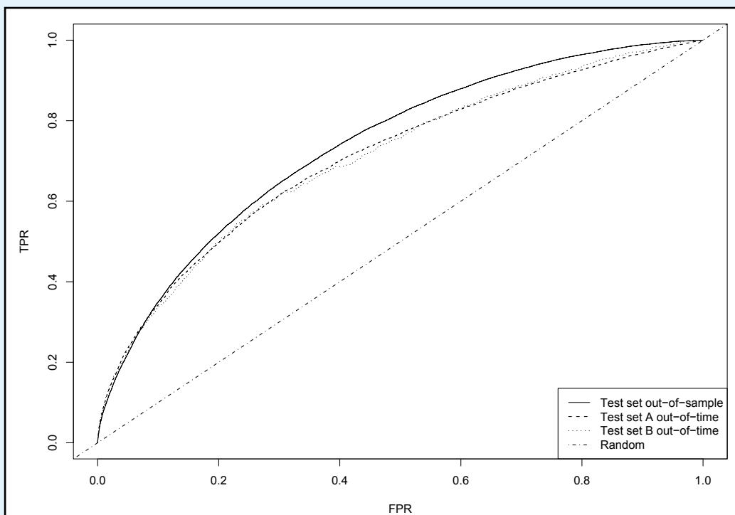
Prediction performance of our model that identifies customers likely to leave the company, compared to random classification of policyholders. Our model is far better than random classification.
