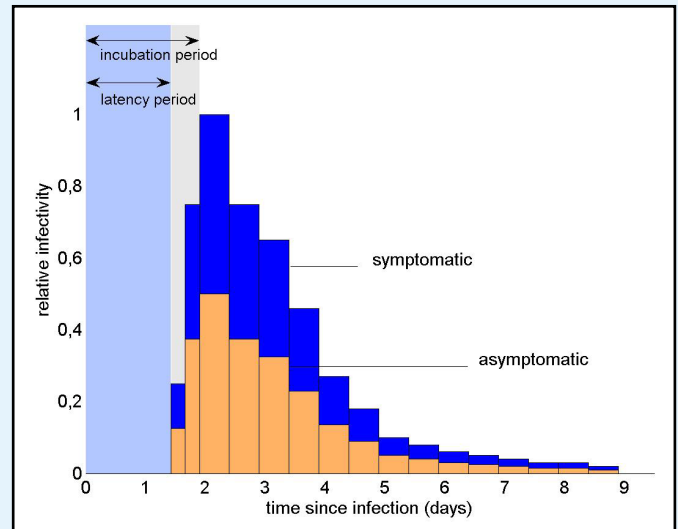
Infectivity profile assumed in the dynamic model for influenza.
